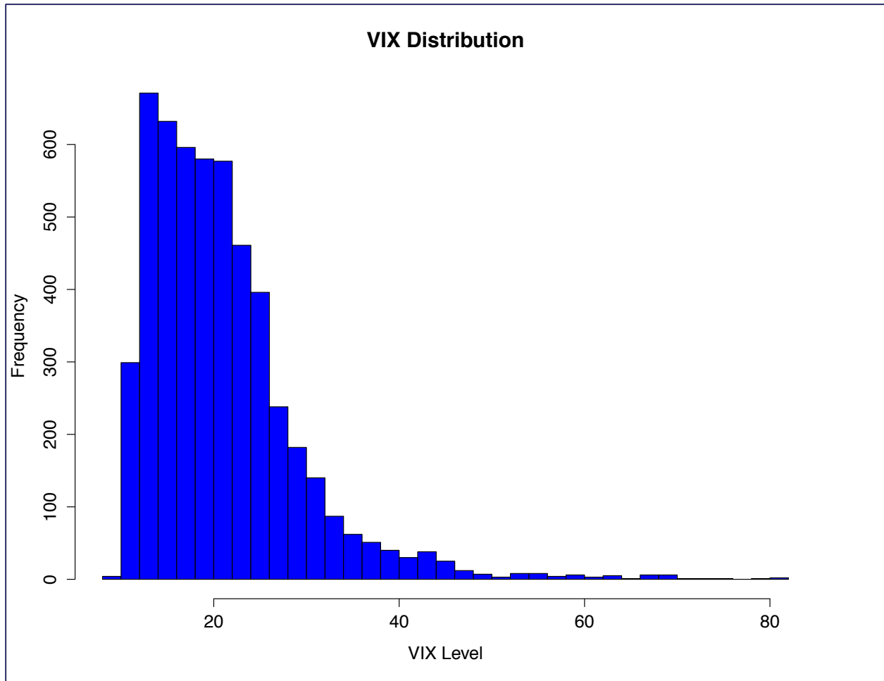
Figure 2 – VIX Histogram
